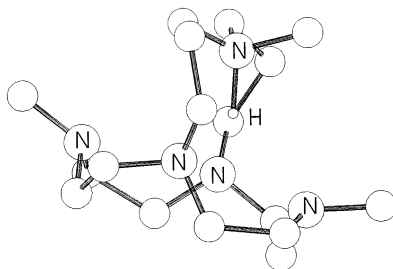
Fig. 19. Drawing of the cation [H(113)]^+ . The atomic coordinates have been taken from Ref. [209].
