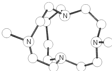
Fig. 20. Drawing of the cation [H(117)]^+ . The atomic coordinates have been taken from Ref. [213].
