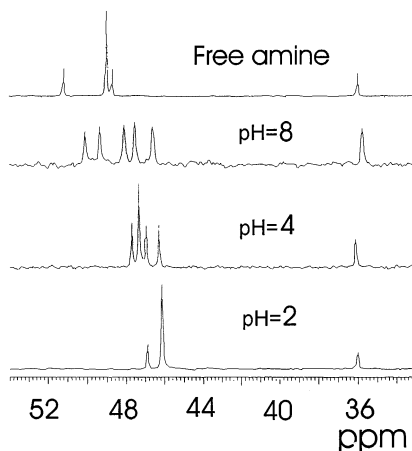
Fig. 9. ^{13}\text{C} -NMR spectra of (26) at different pH values.
