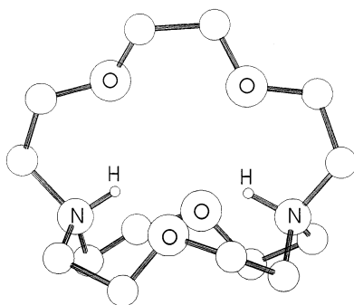
Fig. 17. Drawing of the diprotated cation [\text{H}_2(\text{101})]^{2+} . The atomic coordinates have been taken from Ref. [200].
