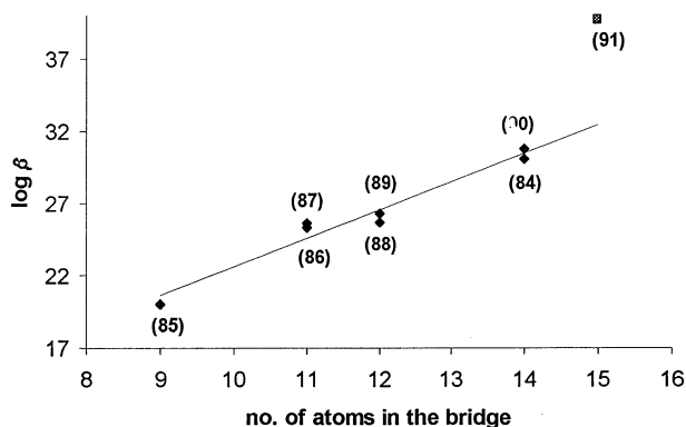
Fig. 15. Representation of the overall basicities ( \text{log } \beta = \sum \text{log } K_i ) of cyclophanes ( 84–91 ) vs. the number of atoms in the bridge.
