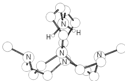
Fig. 18. Drawing of the cation [H(108)]^+ . The atomic coordinates have been taken from Ref. [204].
