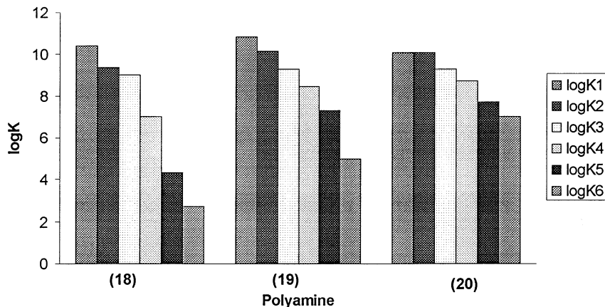
Fig. 3. Bar diagram of the logarithms of the stepwise protonation constants ( \log K ) of hexaamines (18–20).
